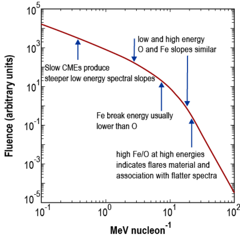
Figure II.6.1: Arbitrary O spectrum summarizing key results in terms of the SEP Band-parameters and their relationships with CME speeds and Fe/O ratios, taken from Desai et al. (2015).
