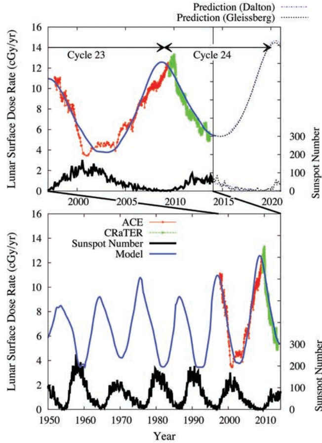
Figure II.1.3. Evolving and increasingly hazardous radiation levels in space. (top) ACE dose rates (red) are based on fits to CRIS spectra; CRaTER measurements (green) from the zenith-facing D1/D2 detectors are used as proxies for lens dose rates behind 0.3 g/cm 2 Al shielding. The sunspot number predictions (the lower black and blue dashed lines) show two cases based on a Gleissberg-like and a Dalton-like minimum, the results of which are similar. The dose predictions (solid blue line and the upper black and blue dashed lines) are from a sunspot-based model of the heliospheric magnetic field and the correlated variation in modulation of GCRs. The ACE data, CRaTER data, and model results are projected to the lunar surface. (bottom) Same as top panel but for a longer time span.
