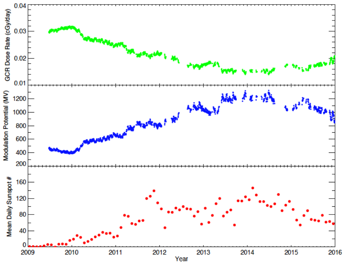
Figure II.3.1. Computed modulation potential over the course of the LRO mission, computed from GCR dose rates (also plotted) using EMMREM-generated lookup tables. The plot extends from the protracted solar minimum of solar cycle 23 to the weak maximum of cycle 24. The average daily sunspot number is provided by the Solar Influences Data Analysis Center is plotted to provide context within the solar cycle.
