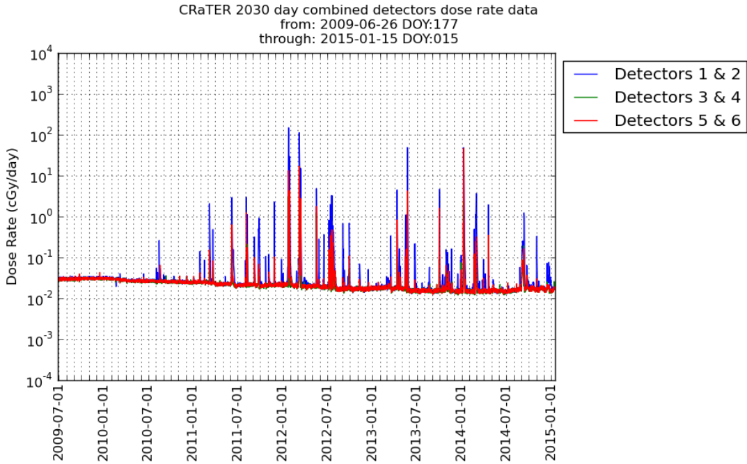
Figure II.1.2. Dose Rates over time through the quantify radiation hazards that damage tissue, materials, and chemically change materials such as lunar regolith.
