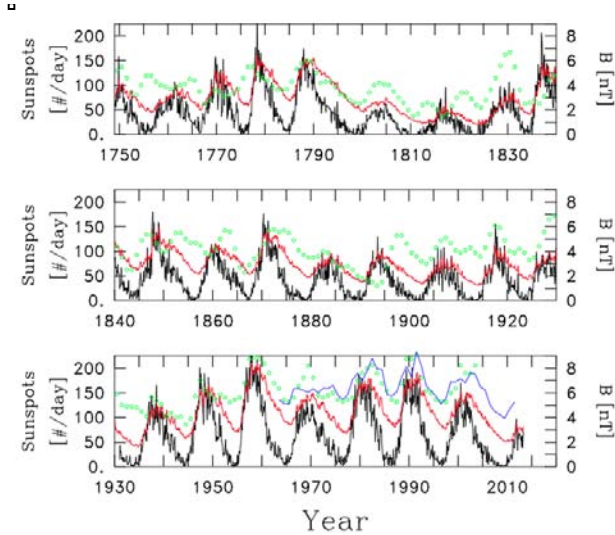
Figure II.1.1: (black) Monthly ave SSN. (red) Predicted Parker comp. of the HMF intensity. (green) Yearly ave HMF intensity derived from ^{10}\text{Be} data. (blue) Measured yearly averages of HMF intensity (Smith et al. [2013]) from the Omni2 data.
