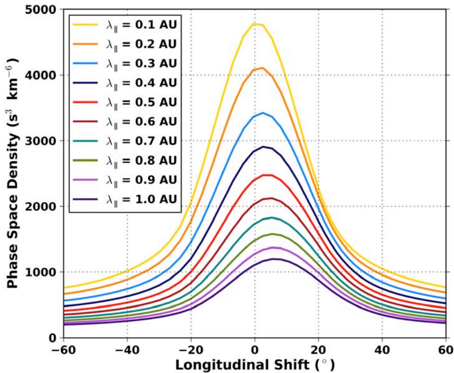
Figure II.4.1. Simulated phase space density of helium pickup ions in the reference frame of STEREO/PLASTIC with limitations by the instrument's acceptance angles and averaged over the energy range of 1.5 < w < 2.0 , where w is the ion speed to solar wind speed ratio. The longitudinal shift for parallel scattering mean free paths of 0.1 AU to 1 AU are shown.
